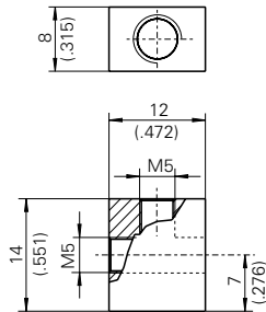
T-piece (PT-300-M5)
