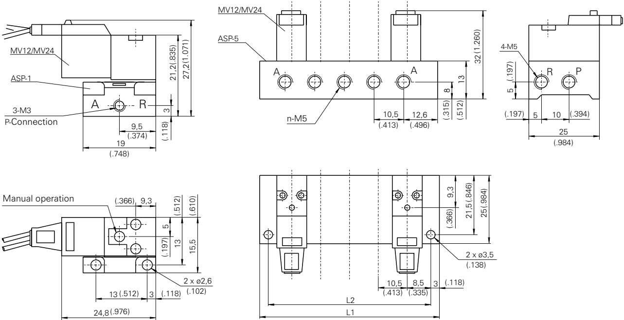
Single Connection Plate (ASP-1)
