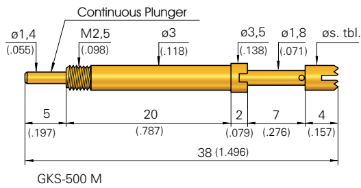
GKS-500 M
